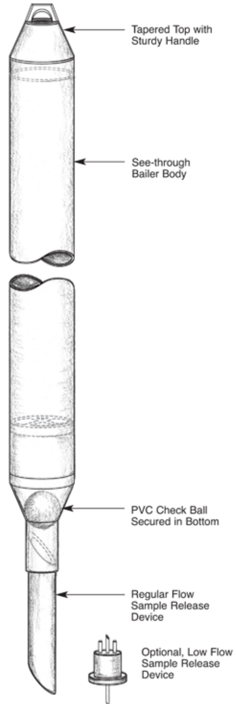
Model 428 Disposable, Translucent Bailer
